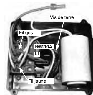
Raccordement 115 Vc.a.
