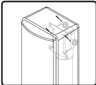
9. Position speaker in desired orientation and tighten all 3 nuts to secure.
