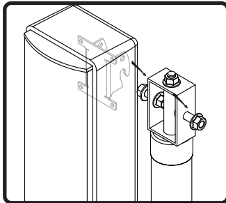
6. Slide speaker with mounting bracket attached onto the Yoke assembly and loosely secure nuts.
