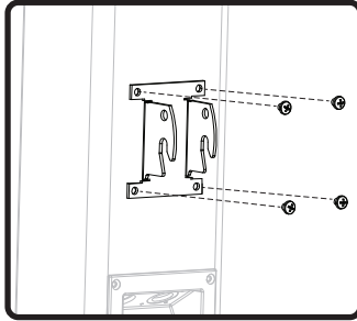
2. Using supplied bolts, attach included mounting bracket to rear of speaker either on the top or bottom of the cabinet depending on the application. WARNING: Do not exceed 100 in-lbs when installing bolts in threaded inserts.
