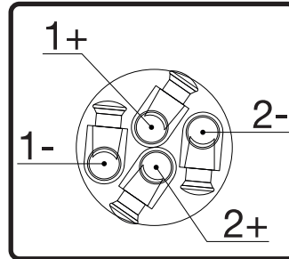
7. Wiring the SpeakOn cable (not included): Wire positive speaker input (+) to SpeakOn +1 terminal and negative speaker input (-) to SpeakOn -1 terminal. Use SpeakOn 2 terminals (+ & -) for daisy-chaining additional speakers.
