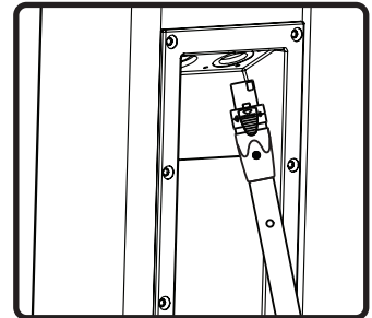
8. Insert the end of the SpeakOn cable into the SpeakOn input connector, and twist to lock.
